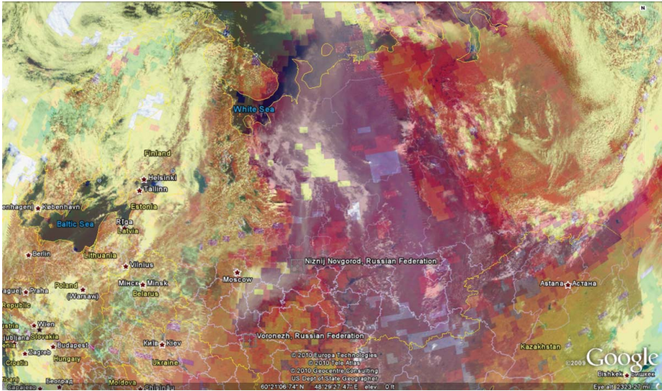
FIGURE 4. Image of Atmospheric Infrared Sounder visible wavelength radiance data (foreground), showing clouds and smoke from Russian wildfires, and overlying CO concentrations (background). Dark red indicates CO concentrations higher than 120 ppb. (Color figure available online).
