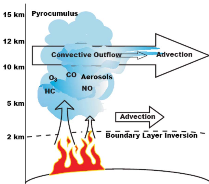
FIGURE 1. Schematic showing the injection of biomass burning emissions into atmospheric layers and their subsequent long range transport in the upper atmosphere. (Color figure available online).
